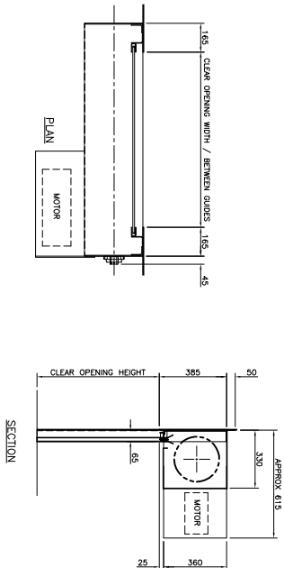
RH SHUTTER – ABOVE 1500mm HIGH
