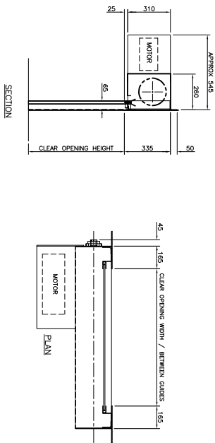
LH SHUTTER – UP TO 1500mm HIGH
