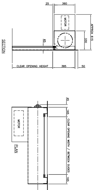
LH SHUTTER – ABOVE 1500mm HIGH
