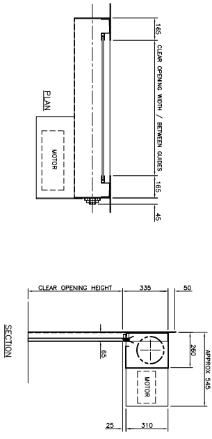
RH SHUTTER – UP TO 1500mm HIGH
