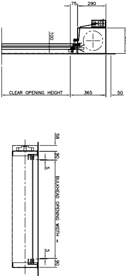
RANGE 1 c/w MAGNET
