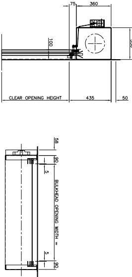
RANGE 2 c/w MAGNET
