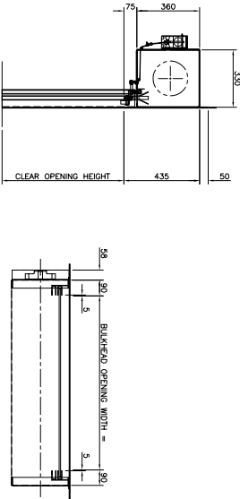
RANGE 2 c/w FUSIBLE LINK & MAGNET
