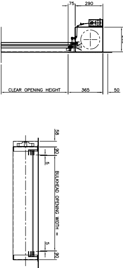
RANGE 1 c/w FUSIBLE LINK & MAGNET
