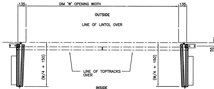
PLAN ON DOORS OPEN
