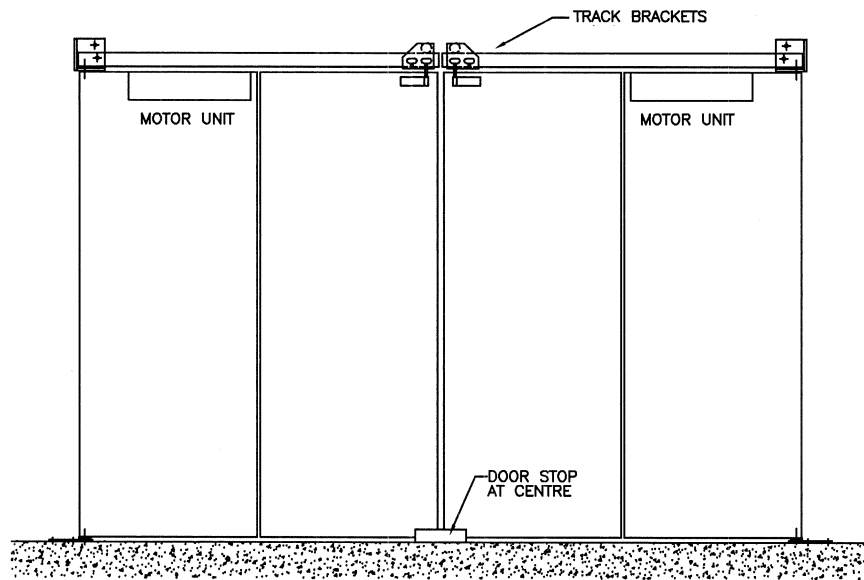
ELEVATION FROM INSIDE (DOORS CLOSED)
