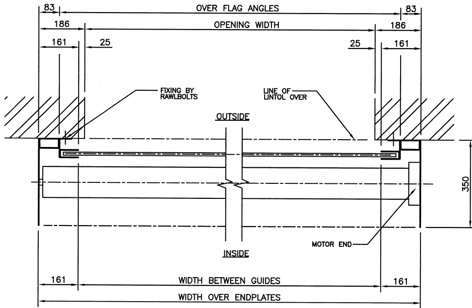
SECTIONAL PLAN
