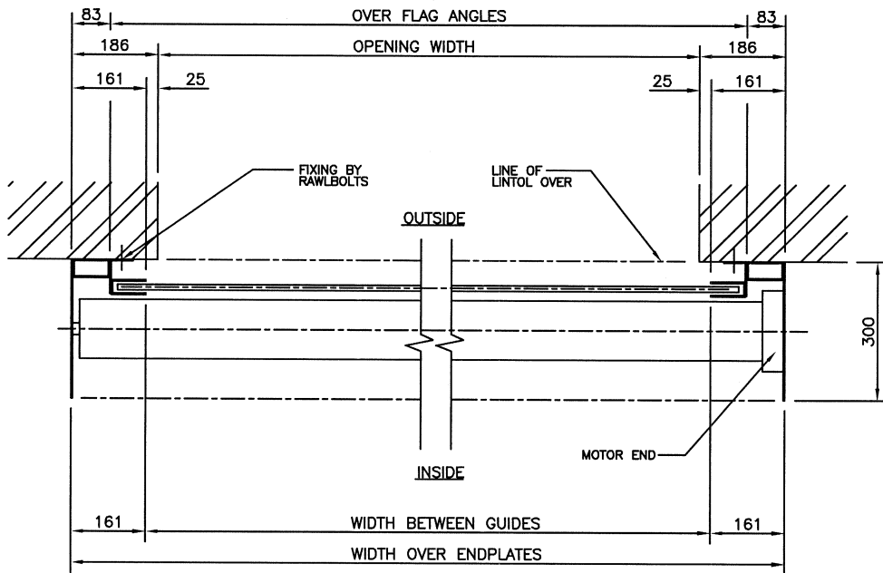
SECTIONAL PLAN
