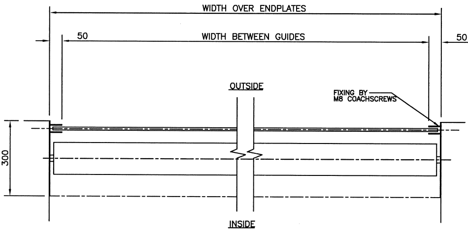
SECTIONAL PLAN
