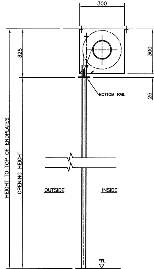
SECTION
