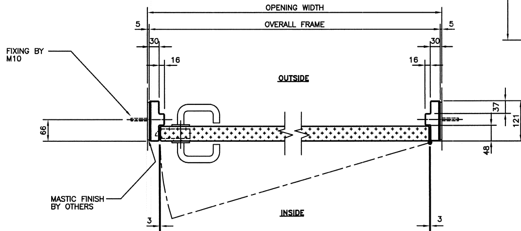
SECTIONAL PLAN
