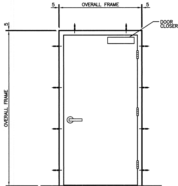
ELEVATION FROM INSIDE
