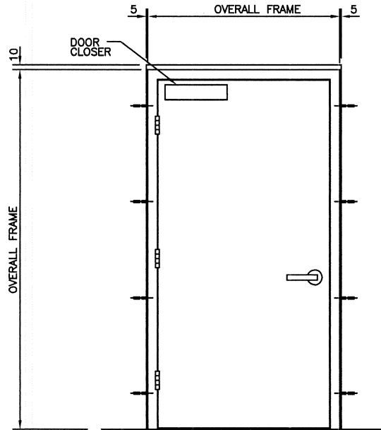
ELEVATION FROM INSIDE
