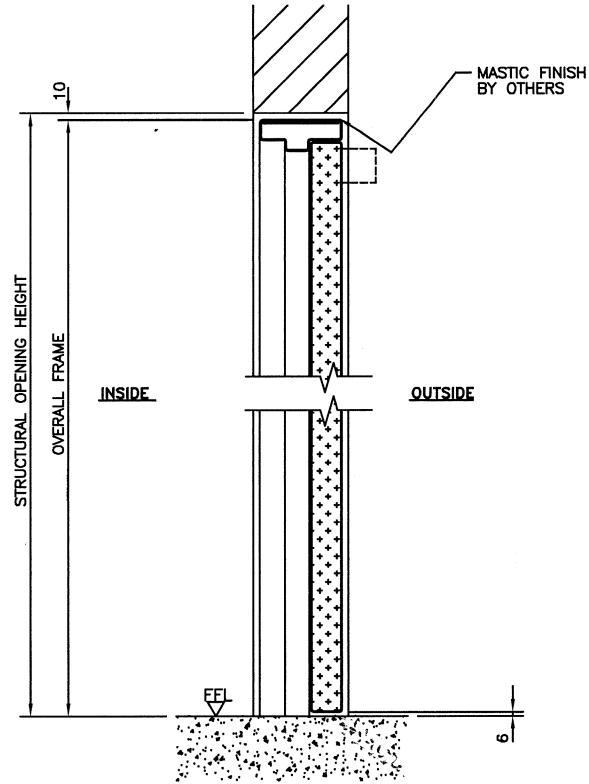
SECTION
