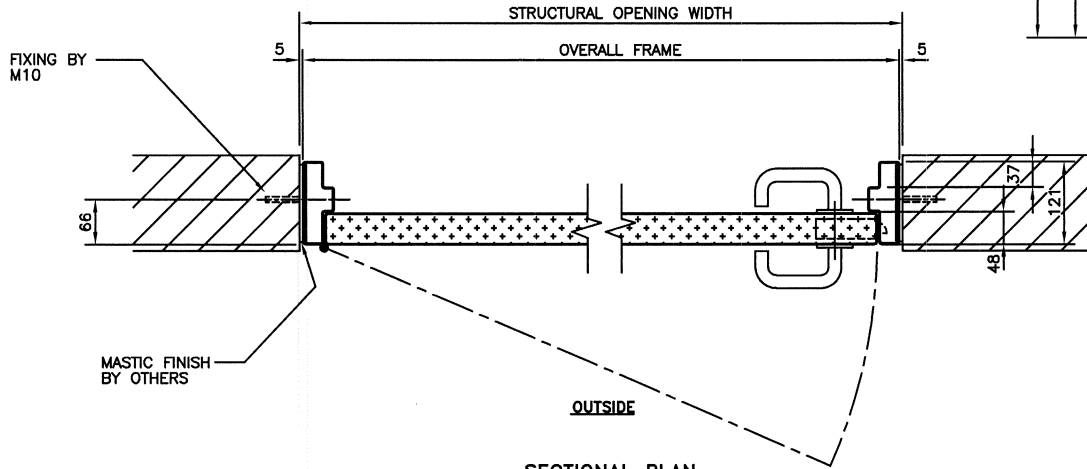
SECTIONAL PLAN
