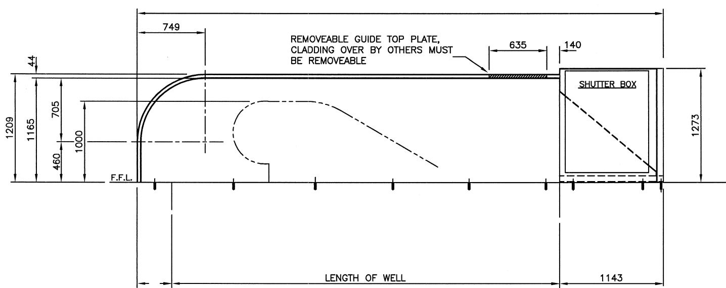
SECTIONAL ELEVATION
