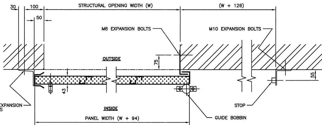
SECTIONAL PLAN
