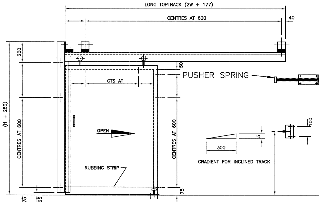
ELEVATION FROM INSIDE
