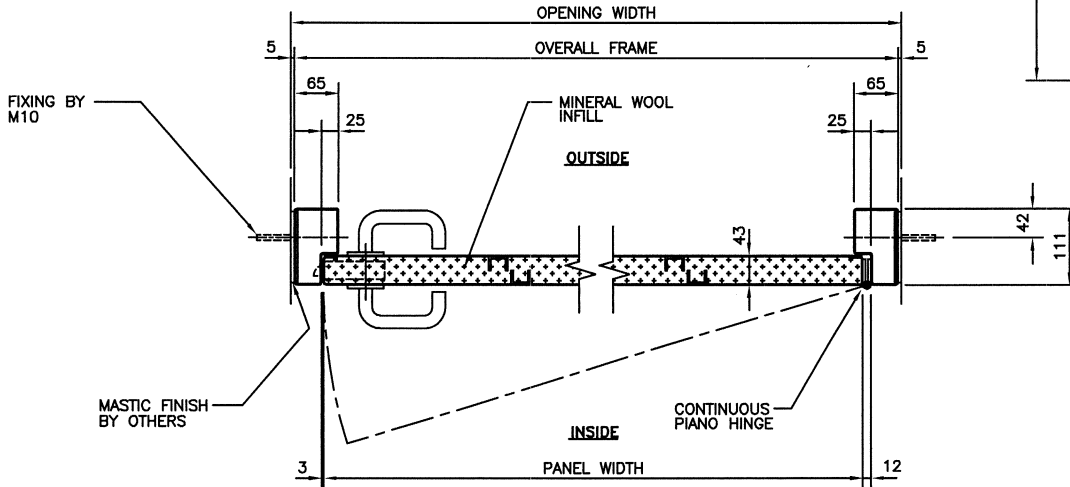
SECTIONAL PLAN
