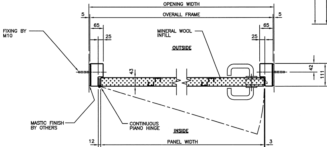
SECTIONAL PLAN
