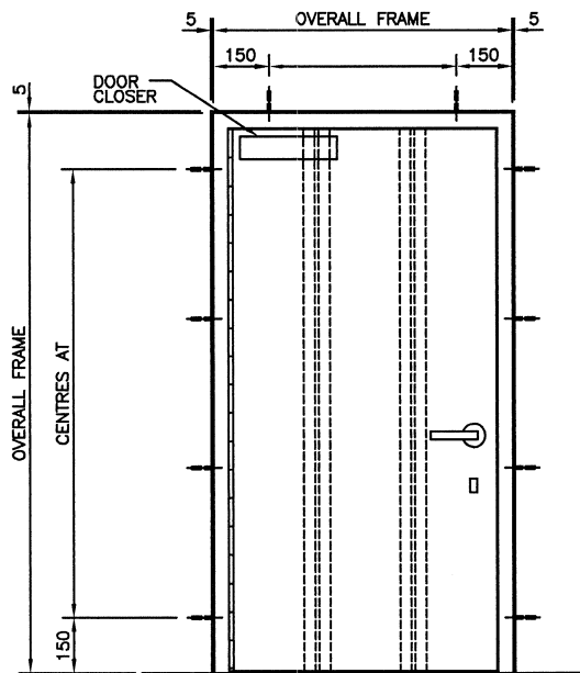
ELEVATION FROM INSIDE
