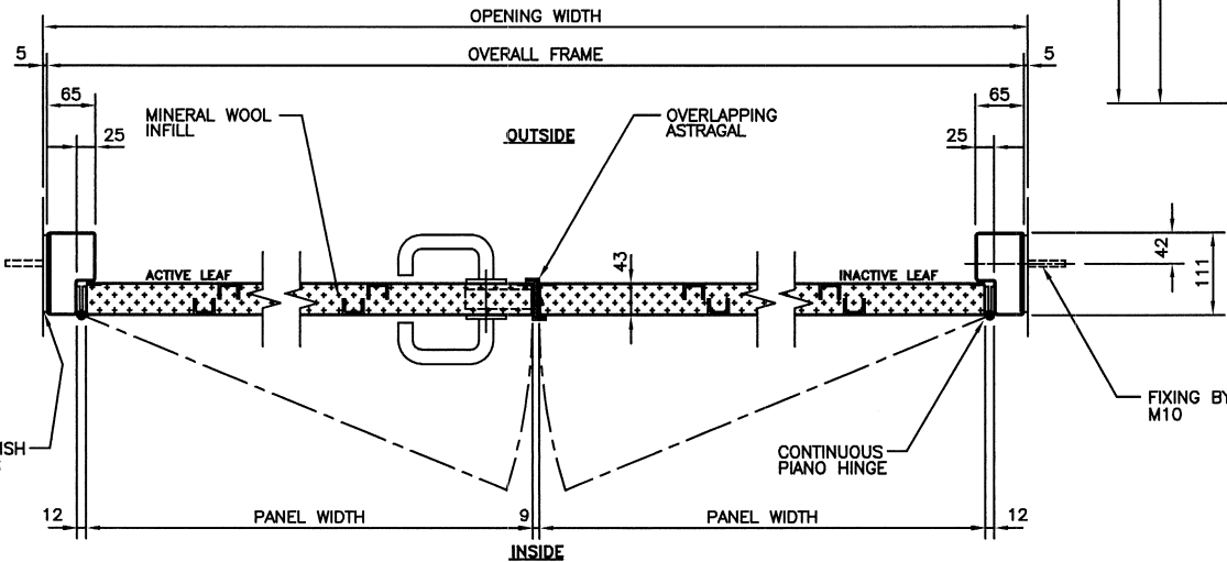
SECTIONAL PLAN
