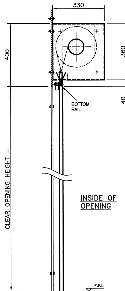
SECTION ON 'A'
